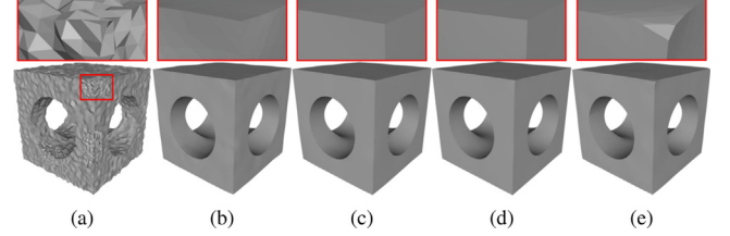
Fig. 5. Denoising results for different \lambda with other parameters fixed. From left to right: noisy input ( \sigma = 0.15\bar{l}_e ), and results with \lambda = 0.01, 0.4, 0.7, 10 .
